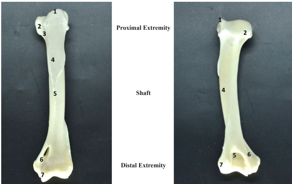
Figure 7. Cranial view of left humerus: 1, Greater tubercle; 2, Lesser tubercle; 3, Neck; 4, Crest of lesser tubercle; 5, Shaft; 6, Supracondyloid foramen; 7, Medial condyle.
