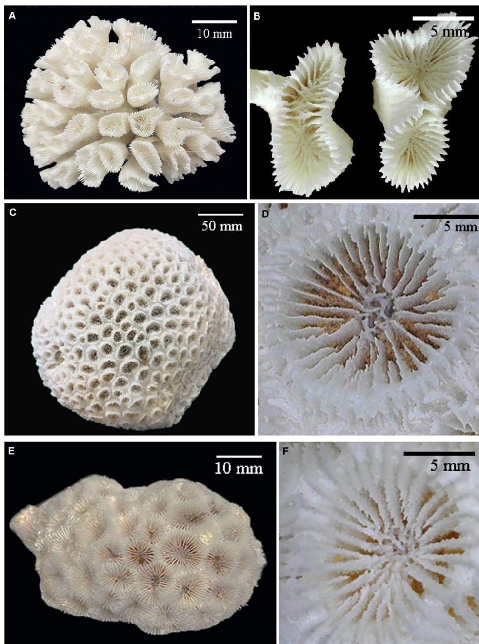
Figure 18. A–B, Caulastrea echinulata (Milne Edwards and Haime, 1848); C–D Dipsastraea matthaii (Vaughan, 1918); E–F, Dipsastraea speciosa (Dana, 1846). A, C, E, colony fragment; B, D, F, septa and corallite.
