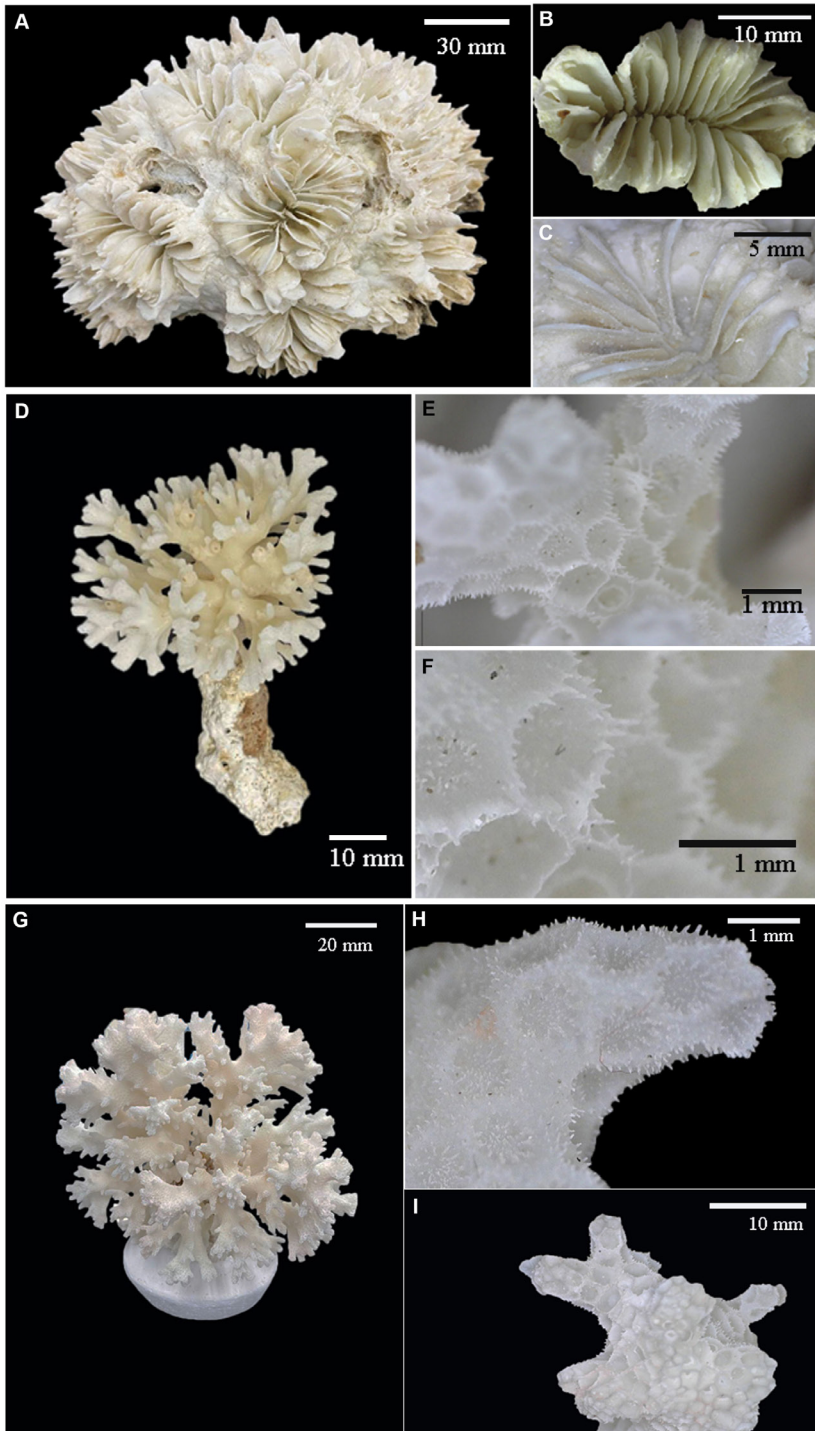
Figure 23. A–C, Plerogyra sinuosa (Dana, 1846), colony; (b,c) Corallite valley with a large septa; (d) Pocillopora aliciae Schmidt–Roach, Miller and Andreakis, 2013, colony fragment; (e,f) Corallite; (g) Pocillopora damicornis (Linnaeus, 1758), colony fragment; (h,i) Corallite.
