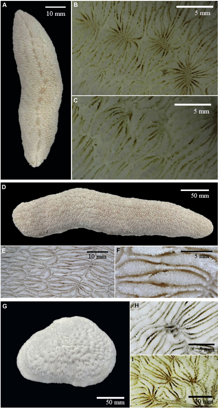
Figure 15. A–F, Herpolitha limax (Esper, 1792), G–I, Sandalolitha robusta (Quelch, 1886). .A, D, G, colony fragment; E, F, septa and axial valley; C, costa between corallite; E, F, H, septa between corallite.
