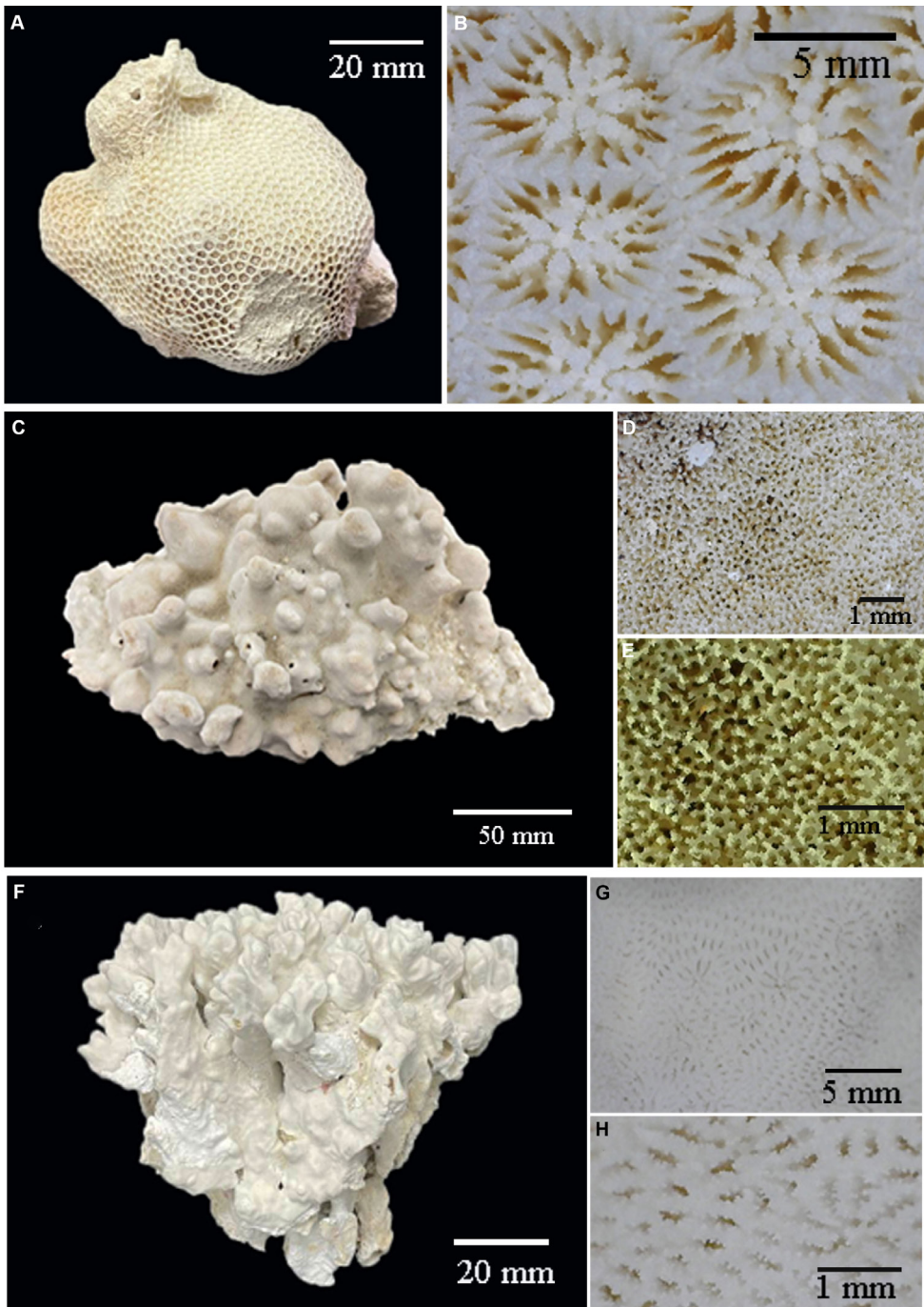
Figure 25. A–B, Goniopora djiboutiensis Vaughan, 1907; C–E, Porites rus (Forskal, 1775); Psammocora contigua (Esper, 1794). A, C, F, colony fragment; B, G, H, septa and corallite; E, F, coralli
