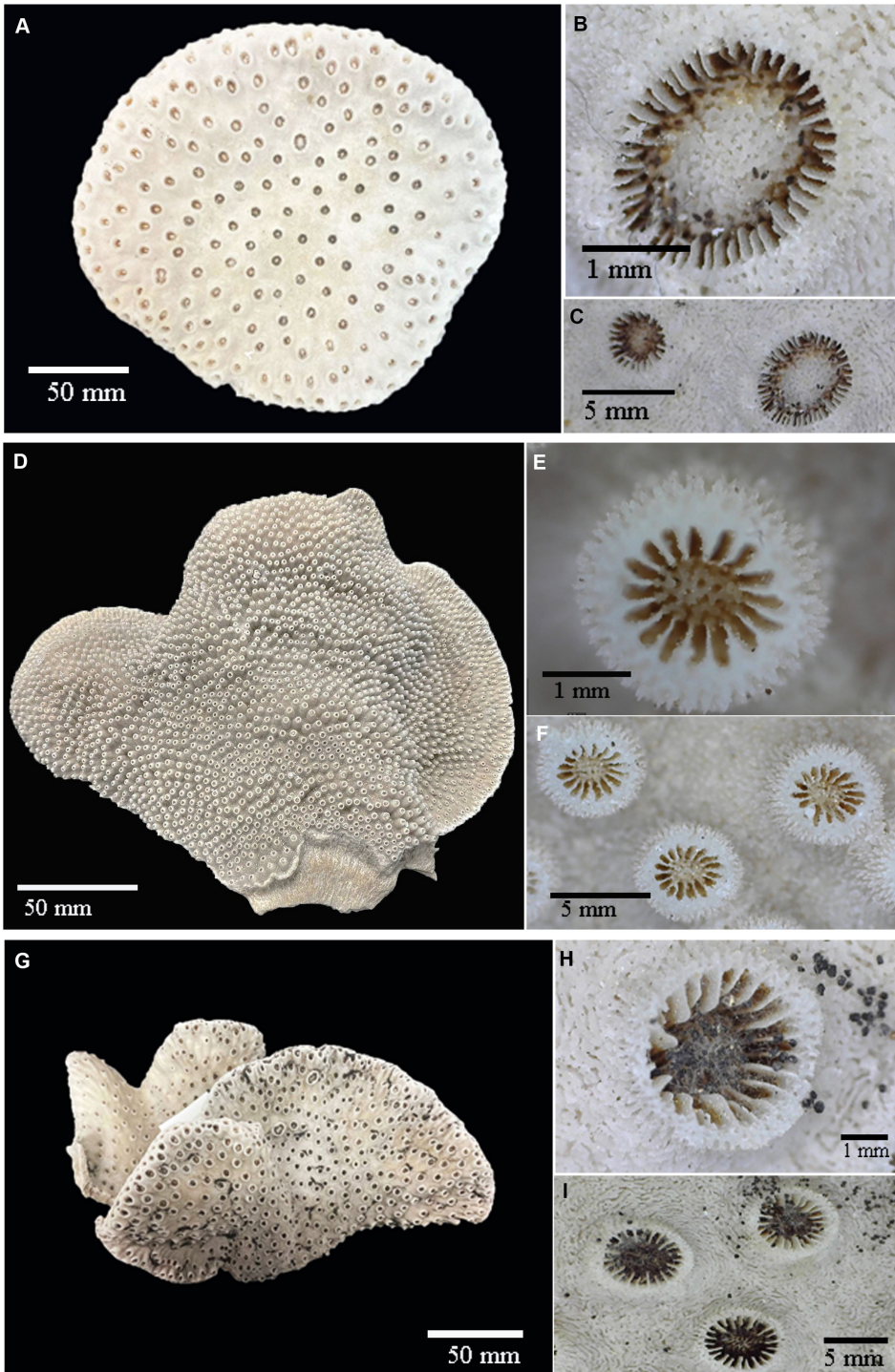
Figure 12. A–C, Duncanopsammia peltata (Esper, 1790); D–F, Turbinaria mesenterina (Lamarck, 1816); G–I, Turbinaria reniformis Bernard, 1896. A, D, G, colony fragment; B, C, E, F, H, I
