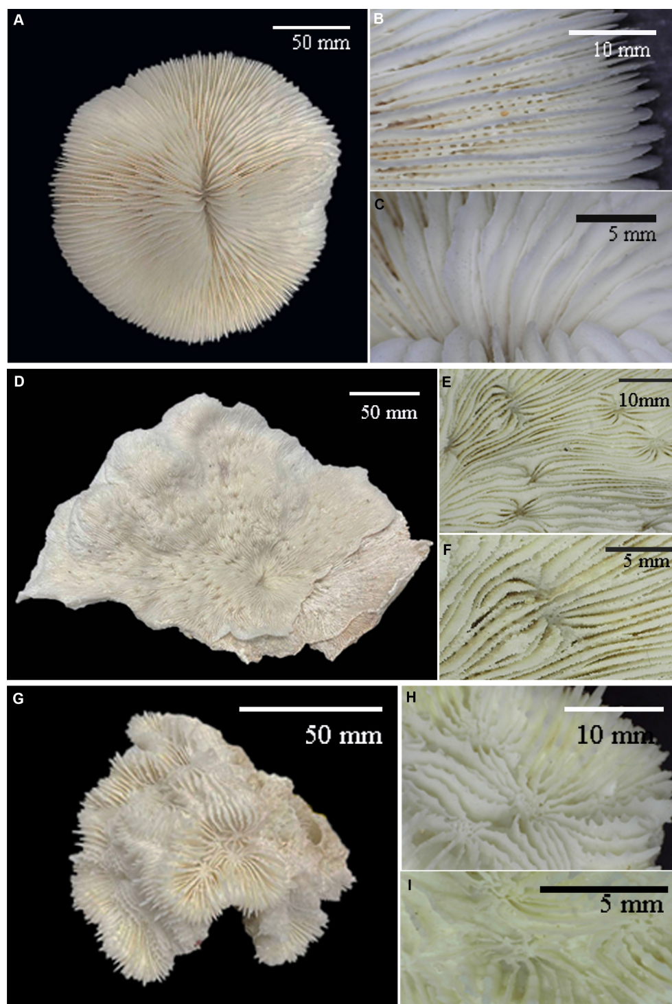
Figure 16. A–C, Litophyllon concinna (Verrill, 1864), D–F, Lithophyllon undulatum Rehberg, 1892; G–I Lobophyllia hataii Yabe, Sugiyama & Eguchi, 1936. A, D, G, colony fragment; B, septa teeth; C, mouth; E, septa along corallite; H, I septa combined with corallite.
